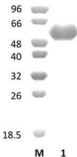
Figure 1. SDS-PAGE analysis of BtFuc29A (GH29) was conducted in (Lane 1), employing a 14% polyacrylamide gel. The enzyme exhibits a band corresponding to a molecular weight of approximately 63,28 kDa. Lane M contains a Protein Marker for reference.
