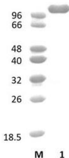
Figure 1. SDS-PAGE analysis of BtLac2C (GH2) was conducted in (Lane 1), employing a 14% polyacrylamide gel. The enzyme exhibits a band corresponding to a molecular weight of approximately 124,4 kDa. Lane M contains a Protein Marker for reference.
