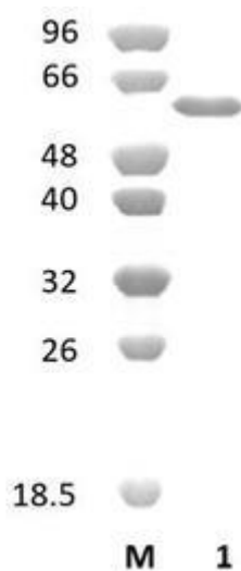
Figure 1. SDS-PAGE analysis of CsXyl39A (GH39) was conducted in (Lane 1), employing a 14% polyacrylamide gel. The enzyme exhibits a band corresponding to a molecular weight of approximately 60,27 kDa. Lane M contains a Protein Marker for reference.
