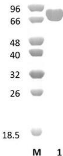
Figure 1. SDS-PAGE analysis of EcGus2A (GH2) was conducted in (Lane 1), employing a 14% polyacrylamide gel. The enzyme exhibits a band corresponding to a molecular weight of approximately 70,54 kDa. Lane M contains a Protein Marker for reference.
