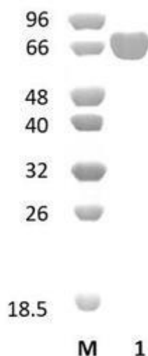
Figure 1. SDS-PAGE analysis of EcSqa31A (GH31) was conducted in (Lane 1), employing a 14% polyacrylamide gel. The enzyme exhibits a band corresponding to a molecular weight of approximately 79,37 kDa. Lane M contains a Protein Marker for reference.
