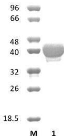
Figure 1. SDS-PAGE analysis of RaMos130A (GH130) was conducted in (Lane 1), employing a 14% polyacrylamide gel. The enzyme exhibits a band corresponding to a molecular weight of approximately 40,40 kDa. Lane M contains a Protein Marker for reference.
