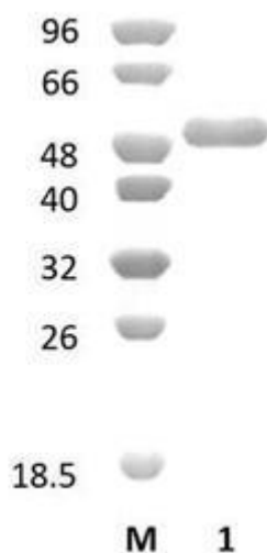
Figure 1. SDS-PAGE analysis of BtPgl28A (GH28) was conducted in (Lane 1), employing a 14% polyacrylamide gel. The enzyme exhibits a band corresponding to a molecular weight of approximately 50,95 kDa. Lane M contains a Protein Marker for reference.
