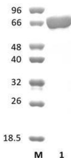
Figure 1. SDS-PAGE analysis of B/Hex20A (GH20) was conducted in (Lane 1), employing a 14% polyacrylamide gel. The enzyme exhibits a band corresponding to a molecular weight of approximately 74,88 kDa. Lane M contains a Protein Marker for reference.
