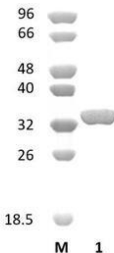
Figure 1. SDS-PAGE analysis of EmAcp18A (GH18) was conducted in (Lane 1), employing a 14% polyacrylamide gel. The enzyme exhibits a band corresponding to a molecular weight of approximately 35,36 kDa. Lane M contains a Protein Marker for reference.
