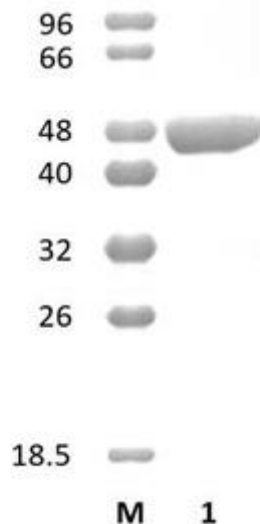
Figure 1. SDS-PAGE analysis of BaAcp18A (CBM50-CBM50-GH18) was conducted in (Lane 1), employing a 14% polyacrylamide gel. The enzyme exhibits a band corresponding to a molecular weight of approximately 50,26 kDa. Lane M contains a Protein Marker for reference.
