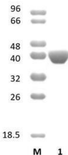
Figure 1. SDS-PAGE analysis of SpAcp73A (GH73) was conducted in (Lane 1), employing a 14% polyacrylamide gel. The enzyme exhibits a band corresponding to a molecular weight of approximately 40,79 kDa. Lane M contains a Protein Marker for reference.
