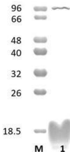
Figure 1. SDS-PAGE analysis of LpAcp73A (GH73) was conducted in (Lane 1), employing a 14% polyacrylamide gel. The enzyme exhibits a band corresponding to a molecular weight of approximately 81,65 kDa. Lane M contains a Protein Marker for reference.
