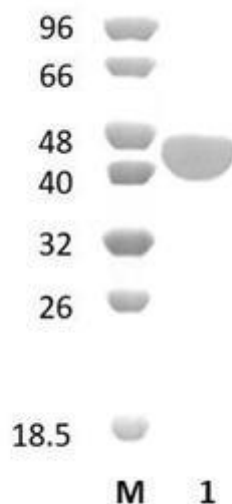
Figure 1. SDS-PAGE analysis of BtUgl105A (GH105) was conducted in (Lane 1), employing a 14% polyacrylamide gel. The enzyme exhibits a band corresponding to a molecular weight of approximately 45,32 kDa. Lane M contains a Protein Marker for reference.
