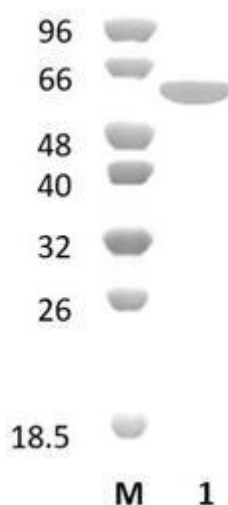
Figure 1. SDS-PAGE analysis of BtPgx28A (GH28) was conducted in (Lane 1), employing a 14% polyacrylamide gel. The enzyme exhibits a band corresponding to a molecular weight of approximately 57,68 kDa. Lane M contains a Protein Marker for reference.
