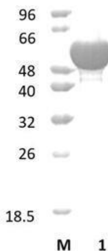
Figure 1. SDS-PAGE analysis of BtPgx28B (GH28) was conducted in (Lane 1), employing a 14% polyacrylamide gel. The enzyme exhibits a band corresponding to a molecular weight of approximately 50,92 kDa. Lane M contains a Protein Marker for reference.
