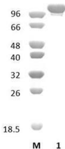
Figure 1. SDS-PAGE analysis of BtGus2A (GH2) was conducted in (Lane 1), employing a 14% polyacrylamide gel. The enzyme exhibits a band corresponding to a molecular weight of approximately 112,7 kDa. Lane M contains a Protein Marker for reference.
