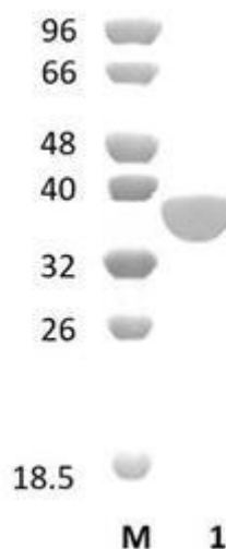
Figure 1. SDS-PAGE analysis of PLam64A (GH64) was conducted in (Lane 1), employing a 14% polyacrylamide gel. The enzyme exhibits a band corresponding to a molecular weight of approximately 37,62 kDa. Lane M contains a Protein Marker for reference.
