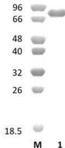
Figure 1. SDS-PAGE analysis of PLam16A (GH16) was conducted in (Lane 1), employing a 14% polyacrylamide gel. The enzyme exhibits a band corresponding to a molecular weight of approximately 81,00 kDa. Lane M contains a Protein Marker for reference.
