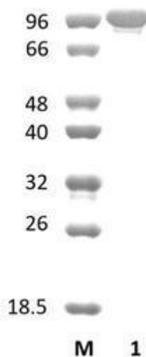
Figure 1. SDS-PAGE analysis of CcXgh44A (GH44-CBM44) was conducted in (Lane 1), employing a 14% polyacrylamide gel. The enzyme exhibits a band corresponding to a molecular weight of approximately 92,09 kDa. Lane M contains a Protein Marker for reference.
