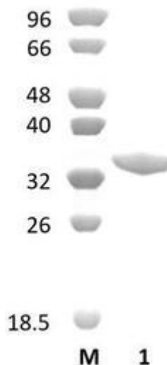
Figure 1. SDS-PAGE analysis of FAcp18A (GH18) was conducted in (Lane 1), employing a 14% polyacrylamide gel. The enzyme exhibits a band corresponding to a molecular weight of approximately 33,13 kDa. Lane M contains a Protein Marker for reference.
