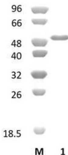
Figure 1. SDS-PAGE analysis of BtAbf43F (GH43-CBM32) was conducted in (Lane 1), employing a 14% polyacrylamide gel. The enzyme exhibits a band corresponding to a molecular weight of approximately 52,59 kDa. Lane M contains a Protein Marker for reference.
