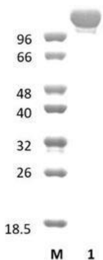
Figure 1. SDS-PAGE analysis of BtRam78B-Kdo33 (CBM67-GH78-GH33) was conducted in (Lane 1), employing a 14% polyacrylamide gel. The enzyme exhibits a band corresponding to a molecular weight of approximately 146,8 kDa. Lane M contains a Protein Marker for reference.
