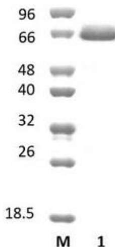
Figure 1. SDS-PAGE analysis of BtPel1D (PL1) was conducted in (Lane 1), employing a 14% polyacrylamide gel. The enzyme exhibits a band corresponding to a molecular weight of approximately 64,77 kDa. Lane M contains a Protein Marker for reference.
