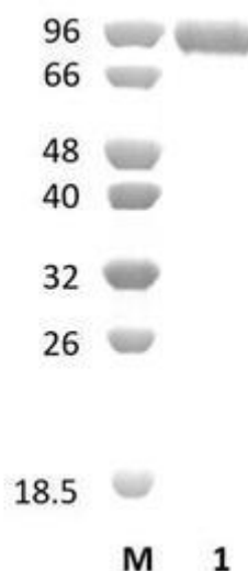
Figure 1. SDS-PAGE analysis of CcXgh74A (GH74-doc-doc) was conducted in (Lane 1), employing a 14% polyacrylamide gel. The enzyme exhibits a band corresponding to a molecular weight of approximately 93,37 kDa. Lane M contains a Protein Marker for reference.
