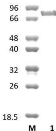
Figure 1. SDS-PAGE analysis of CcBgl3A (GH3) was conducted in (Lane 1), employing a 14% polyacrylamide gel. The enzyme exhibits a band corresponding to a molecular weight of approximately 81,67 kDa. Lane M contains a Protein Marker for reference.
