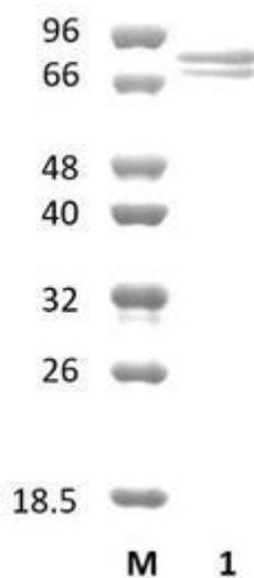
Figure 1. SDS-PAGE analysis of RcCel9E (GH9-CBM3) was conducted in (Lane 1), employing a 14% polyacrylamide gel. The enzyme exhibits a band corresponding to a molecular weight of approximately 79,44 kDa. Lane M contains a Protein Marker for reference.
