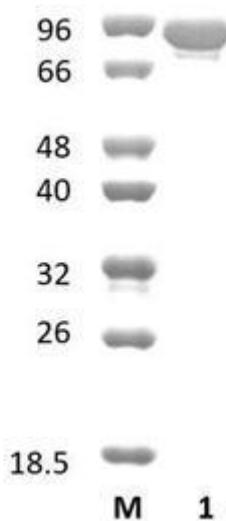
Figure 1. SDS-PAGE analysis of RcCbh48A (GH48) was conducted in (Lane 1), employing a 14% polyacrylamide gel. The enzyme exhibits a band corresponding to a molecular weight of approximately 86,35 kDa. Lane M contains a Protein Marker for reference.
