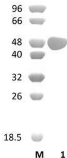
Figure 1. SDS-PAGE analysis of GsArb27A (GH27) was conducted in (Lane 1), employing a 14% polyacrylamide gel. The enzyme exhibits a band corresponding to a molecular weight of approximately 51,71 kDa. Lane M contains a Protein Marker for reference.
