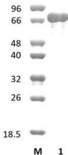
Figure 1. SDS-PAGE analysis of NpAms13A (GH13) was conducted in (Lane 1), employing a 14% polyacrylamide gel. The enzyme exhibits a band corresponding to a molecular weight of approximately 74,43 kDa. Lane M contains a Protein Marker for reference.
