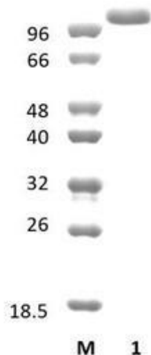
Figure 1. SDS-PAGE analysis of BtMns92B (GH92-GH92) was conducted in (Lane 1), employing a 14% polyacrylamide gel. The enzyme exhibits a band corresponding to a molecular weight of approximately 101,3 kDa. Lane M contains a Protein Marker for reference.
