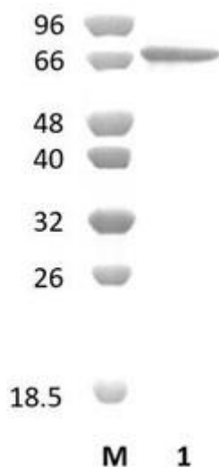
Figure 1. SDS-PAGE analysis of EcAgl13A (CBM34-GH13) was conducted in (Lane 1), employing a 14% polyacrylamide gel. The enzyme exhibits a band corresponding to a molecular weight of approximately 71,26 kDa. Lane M contains a Protein Marker for reference.
