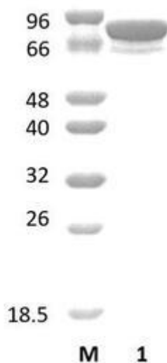
Figure 1. SDS-PAGE analysis of EcAgl63A (GH63) was conducted in (Lane 1), employing a 14% polyacrylamide gel. The enzyme exhibits a band corresponding to a molecular weight of approximately 88,07 kDa. Lane M contains a Protein Marker for reference.
