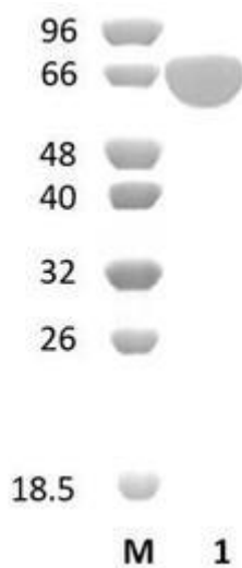
Figure 1. SDS-PAGE analysis of SpLac35A (GH35) was conducted in (Lane 1), employing a 14% polyacrylamide gel. The enzyme exhibits a band corresponding to a molecular weight of approximately 71,04 kDa. Lane M contains a Protein Marker for reference.
