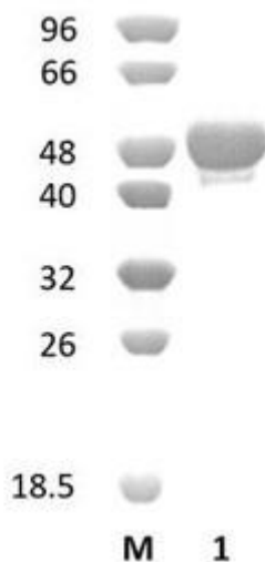
Figure 1. SDS-PAGE analysis of TpAbn43A (GH43) was conducted in (Lane 1), employing a 14% polyacrylamide gel. The enzyme exhibits a band corresponding to a molecular weight of approximately 53,38 kDa. Lane M contains a Protein Marker for reference.
