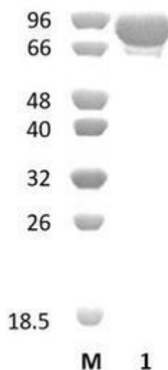
Figure 1. SDS-PAGE analysis of PbXyl3A (GH3) was conducted in (Lane 1), employing a 14% polyacrylamide gel. The enzyme exhibits a band corresponding to a molecular weight of approximately 86,28 kDa. Lane M contains a Protein Marker for reference.
