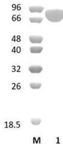
Figure 1. SDS-PAGE analysis of AaLac42A (GH42) was conducted in (Lane 1), employing a 14% polyacrylamide gel. The enzyme exhibits a band corresponding to a molecular weight of approximately 79,88 kDa. Lane M contains a Protein Marker for reference.
