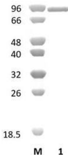
Figure 1. SDS-PAGE analysis of CpOgr65A (GH65) was conducted in (Lane 1), employing a 14% polyacrylamide gel. The enzyme exhibits a band corresponding to a molecular weight of approximately 90,08 kDa. Lane M contains a Protein Marker for reference.
