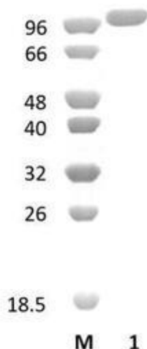
Figure 1. SDS-PAGE analysis of SpHys8A (PL8) was conducted in (Lane 1), employing a 14% polyacrylamide gel. The enzyme exhibits a band corresponding to a molecular weight of approximately 116,4 kDa. Lane M contains a Protein Marker for reference.
