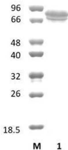
Figure 1. SDS-PAGE analysis of RfXyn10A (CBM22-GH10-Doc) was conducted in (Lane 1), employing a 14% polyacrylamide gel. The enzyme exhibits a band corresponding to a molecular weight of approximately 71,54 kDa. Lane M contains a Protein Marker for reference.
