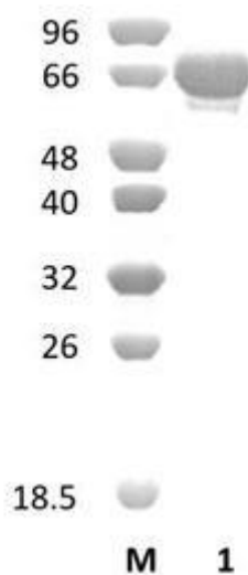
Figure 1. SDS-PAGE analysis of RcMan5A (CBM23-GH5) was conducted in (Lane 1), employing a 14% polyacrylamide gel. The enzyme exhibits a band corresponding to a molecular weight of approximately 67,79 kDa. Lane M contains a Protein Marker for reference.
