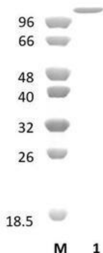
Figure 1. SDS-PAGE analysis of RcXyn10B-Abf43B (CBM22-GH10-CBM22-GH43-CBM6) was conducted in (Lane 1), employing a 14% polyacrylamide gel. The enzyme exhibits a band corresponding to a molecular weight of approximately 135,3 kDa. Lane M contains a Protein Marker for reference.
