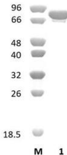
Figure 1. SDS-PAGE analysis of RcXgh44A (GH44-CBM76) was conducted in (Lane 1), employing a 14% polyacrylamide gel. The enzyme exhibits a band corresponding to a molecular weight of approximately 80,28 kDa. Lane M contains a Protein Marker for reference.
