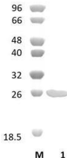
Figure 1. SDS-PAGE analysis of BtRme NC (CE NC) was conducted in (Lane 1), employing a 14% polyacrylamide gel. The enzyme exhibits a band corresponding to a molecular weight of approximately 26,38 kDa. Lane M contains a Protein Marker for reference.
