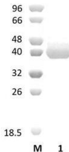
Figure 1. SDS-PAGE analysis of GFP-CBM48 was conducted in (Lane 1), employing a 14% polyacrylamide gel. The enzyme exhibits a band corresponding to a molecular weight of approximately 40,88 kDa. Lane M contains a Protein Marker for reference.
