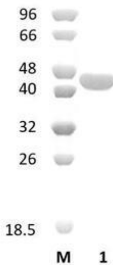
Figure 1. SDS-PAGE analysis of GFP-CBM48 was conducted in (Lane 1), employing a 14% polyacrylamide gel. The enzyme exhibits a band corresponding to a molecular weight of approximately 41,55 kDa. Lane M contains a Protein Marker for reference.
