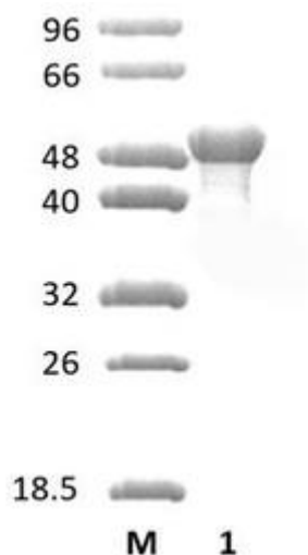
Figure 1. SDS-PAGE analysis of TmXyn10B (GH10) was conducted in (Lane 1), employing a 14% polyacrylamide gel. The enzyme exhibits a band corresponding to a molecular weight of approximately 46,58 kDa. Lane M contains a Protein Marker for reference.
