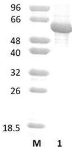
Figure 1. SDS-PAGE analysis of LaLam157A (GH157) was conducted in (Lane 1), employing a 14% polyacrylamide gel. The enzyme exhibits a band corresponding to a molecular weight of approximately 61,43 kDa. Lane M contains a Protein Marker for reference.
