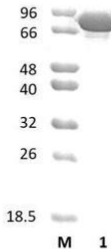
Figure 1. SDS-PAGE analysis of ZgFuc95D (GH95) was conducted in (Lane 1), employing a 14% polyacrylamide gel. The enzyme exhibits a band corresponding to a molecular weight of approximately 90,25 kDa. Lane M contains a Protein Marker for reference.
