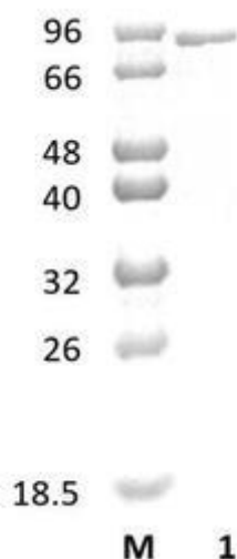
Figure 1. SDS-PAGE analysis of ZgRam78A (CBM67-GH78) was conducted in (Lane 1), employing a 14% polyacrylamide gel. The enzyme exhibits a band corresponding to a molecular weight of approximately 90,83 kDa. Lane M contains a Protein Marker for reference.
