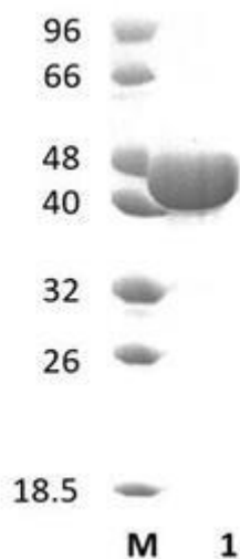
Figure 1. SDS-PAGE analysis of ZgXyn10A (GH10) was conducted in (Lane 1), employing a 14% polyacrylamide gel. The enzyme exhibits a band corresponding to a molecular weight of approximately 42,87 kDa. Lane M contains a Protein Marker for reference.
